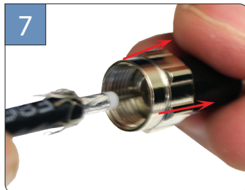
7 Once the center conductor is pressed fully into the pin pull the connector away from the cable. The step up pin and insulator guide will stay with the cable as shown.
