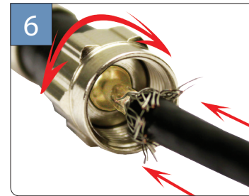
6 Insert cable center conductor into the pin stored within the nut of the connector. Push into the pin while rotating the connector.
