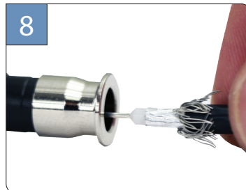
8 Insert the cable into the back of the connector with the step up pin and insulator guide inside the post. Push the connector on while rotating until fully seated.
