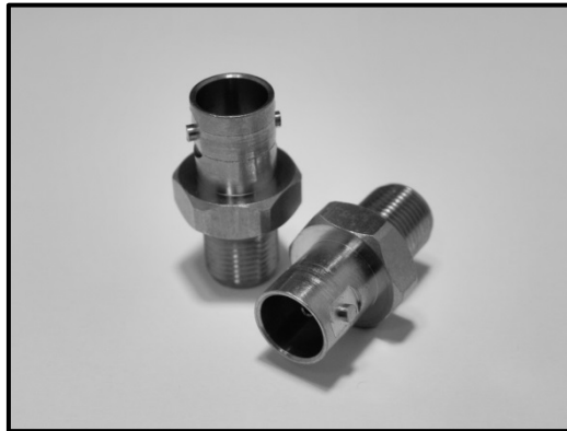
Description: Adaptor, BNC female – F female.
