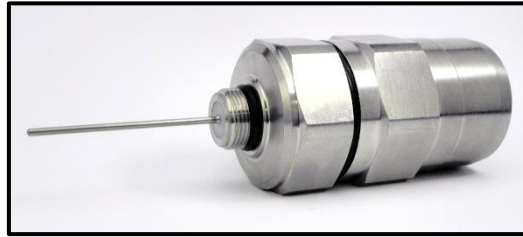
Description: Hardline Connector, R044 – 5/8 male. (Measured with POPE 75 OHM, 37001 Cable. 0.54 m.)
