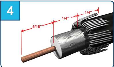
Ensure the cable is prepared to the proper dimensions.
