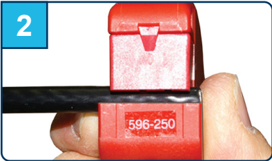
Using a fixed blade with a prep tool in good condition, prepare the cable to 5/16" x 1/4" x 1/4" dimensions. Use the edge of the tool if there is no stop.
