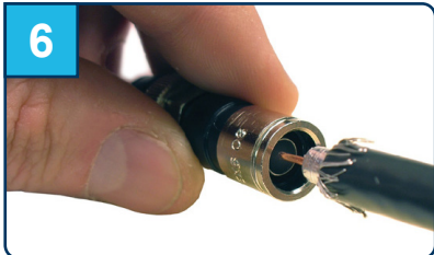
Guide the center conductor and dielectric into the connector post. Insert the cable into the connector until the dielectric is flush within the post.
