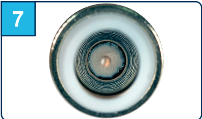
Here you can see the dielectric is flush within the post.
