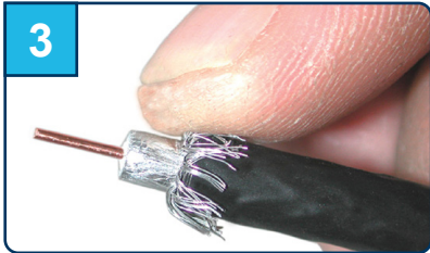
Fold back the braid. If using tri-shield or quad-shield cables, remove the additional foil layer and fold back the remaining braid.
