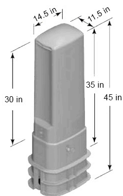
Pedestal FDH
